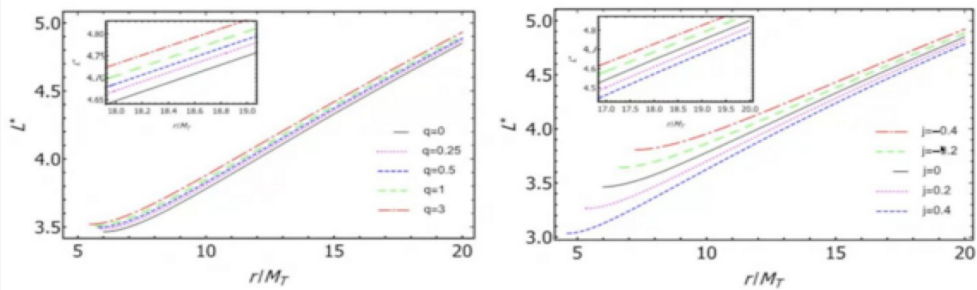
FIG. 3. Angular momentum L^* of test particles versus radial distance r normalized in units of total mass M_T . Left panel: L^* in the q metric for oblate sources ( q > 0 ). Right panel: in the Kerr space-time.
